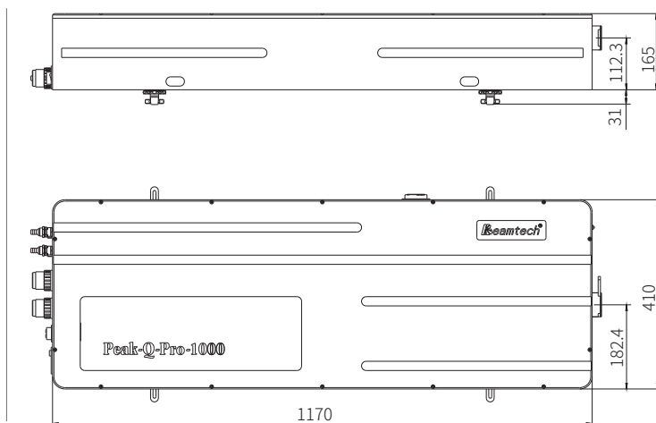
Peak-Q-Pro-1000 激光头
